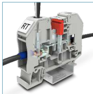
Reihenklemme RT 5
